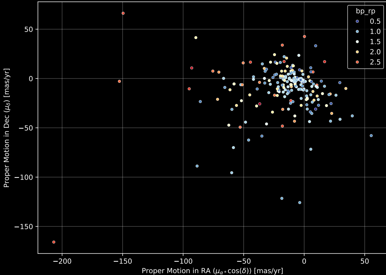
APOGEE DR17 Field: [K2_C1_277+58_btx] Proper Motion Diagram (n= 206)
