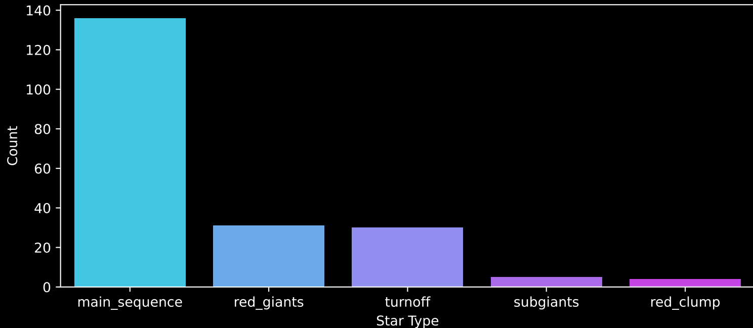
APOGEE DR17 Field: [K2_C1_277+58_btx] Count plot of Star Type
