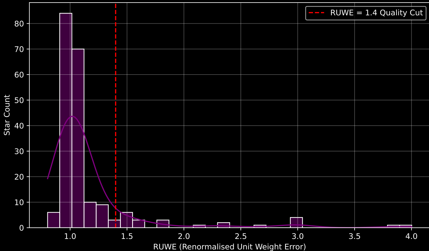
GAPOGEE DR17 Field [K2_C1_277+58_btx] RUWE Distribution (n= 204)
