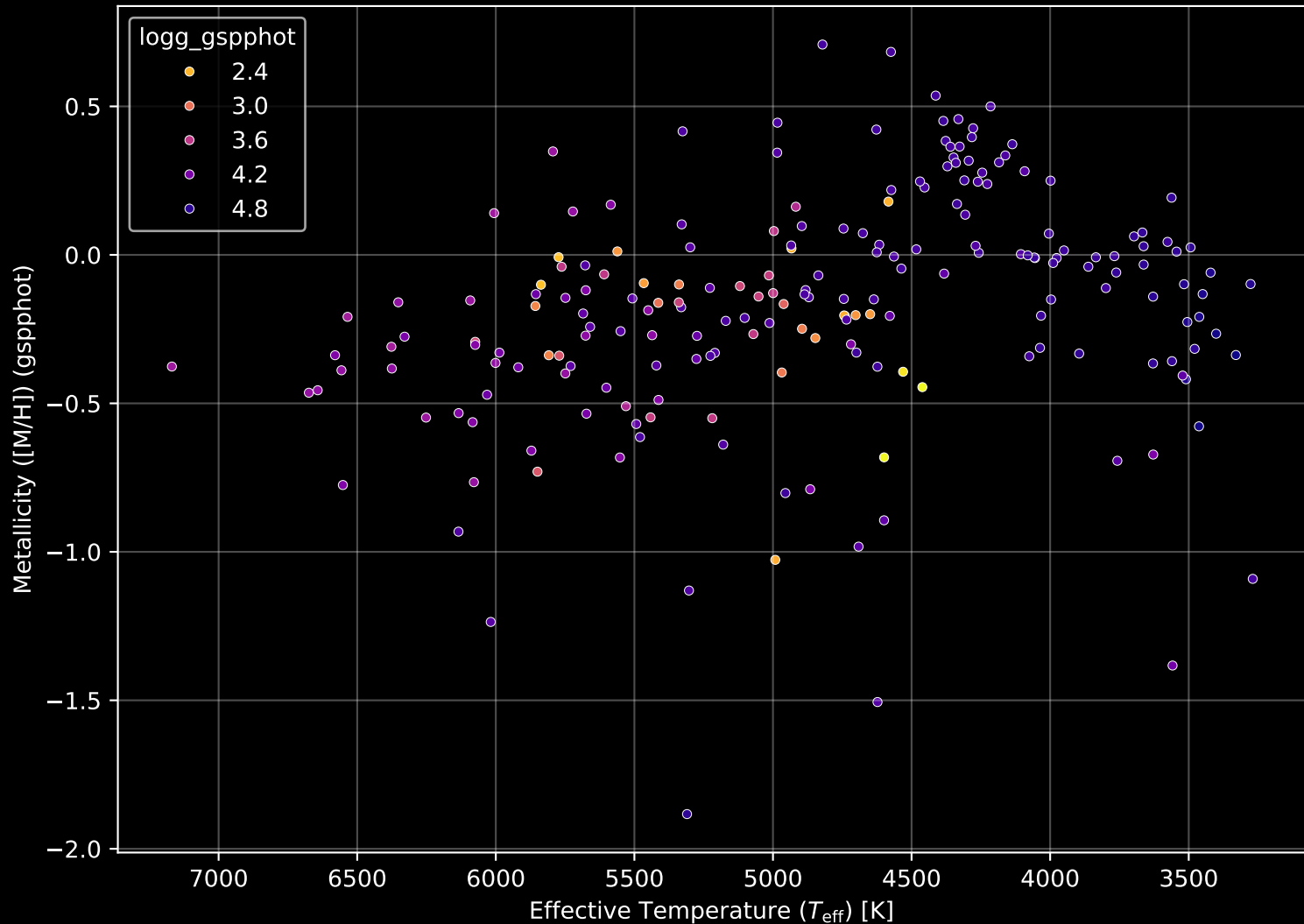
APOGEE DR17 Field: [K2_C1_277+58_btx] Stellar Population Parameters (n= 206)
