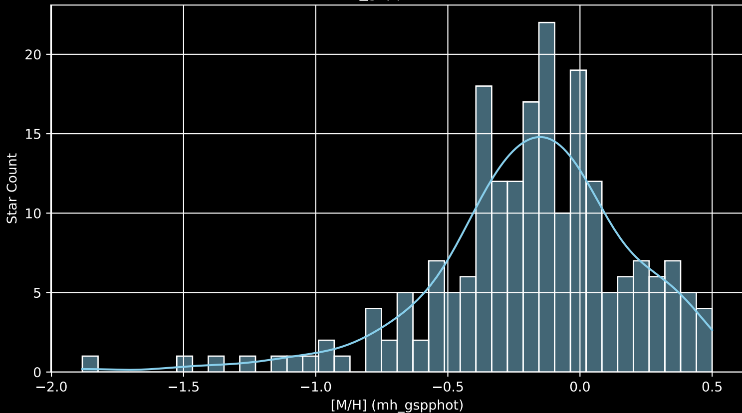
APOGEE DR17 Field: [K2_C1_277+58_btx [M/H] (mh_gspphot) (n= 203)
