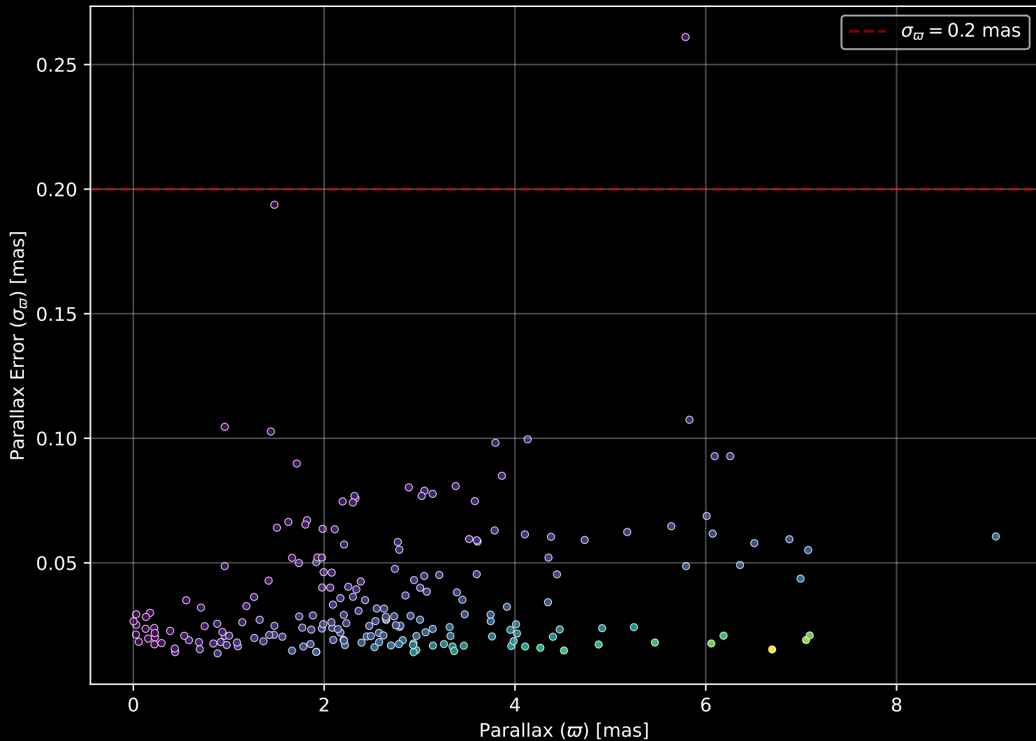
APOGEE DR17 Field: [K2_C1_277+58_btx] Parallax Quality (n= 206)
